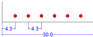
Fig 4, Runway end lights at Vardø airport (ENSS)
