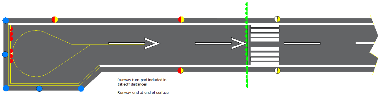
Fig 9, Runway turn pad extension to one side
